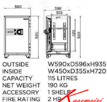
SB40D5 Outside Dimension (WxDxH)[MM.] 590 X 596 X 935 Inside Dimension (WxDxH)[MM.]450 X 355 X 720 Net Weight 190 KG Capacity 115 Litres
