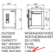
SS2DKN Outside Dimension (WxDxH)[MM.] 344 X 427 X 512 Inside Dimension (WxDxH)[MM.] 217 X 264 X 357 Net Weight 50 KG Capacity 20 Litres
