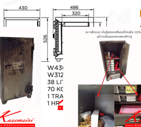
SS70D4OV Outside Dimension [WxDxH][MM.] 430 X 486 X 526 Inside Dimension [WxDxH][MM.] 312 X 320 X 380 Net Weight 70 KG Capacity 38 Litres
