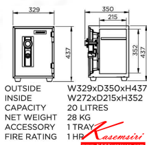
LS2DKN Outside Dimension (WxDxH)[MM.] 329 X 350 X 437 Inside Dimension (WxDxH)[MM.] 272 X 215 X 352 Net Weight 28 KG Capacity 20 Litres
