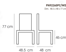
PN92260PC/WD Dim. 48.5 x 48 x 77 cm color : black
