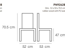
PN92628 Dim. 52 x 53 x 70.5 cm rubber wood with PU seat
