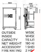
SB40D Outside Dimension (WxDxH)[MM.] 590 X 596 X 935 Inside Dimension (WxDxH)[MM.] 450 X 355 X 720 Net Weight 190 KG Capacity 115 Litres
