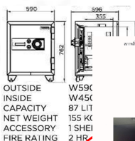
SB30D Outside Dimension (WxDxH)[MM.] 590 X 596 X 762 Inside Dimension (WxDxH)[MM.] 450 X 355 X 547 Net Weight 155 KG Capacity 87 Litres
